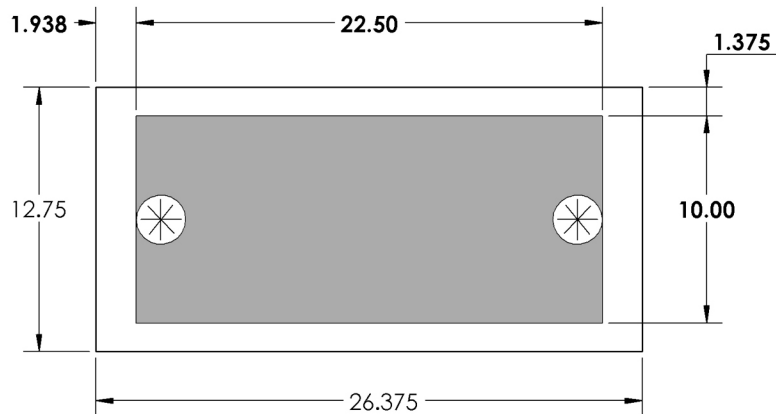
Console Top Removable Panel Cutout
