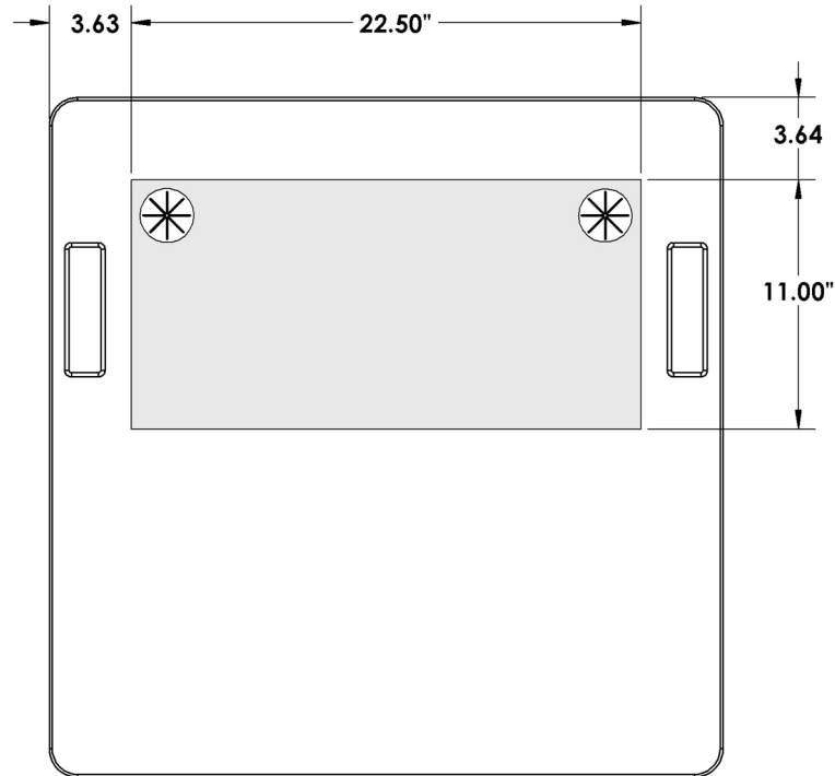
Work Surface Cutout
